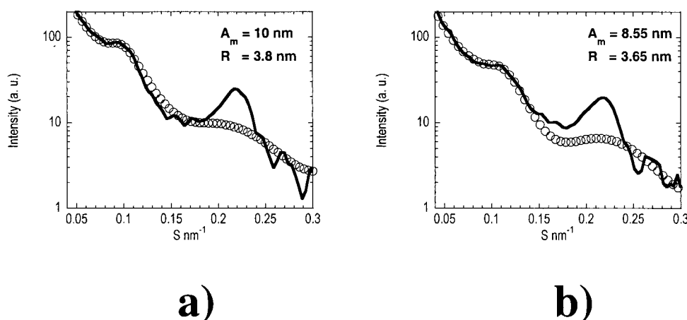
FIGURE 6 One-dimensional equatorial intensity profiles extracted from the SAXS patterns of the human hair fiber continuously stretched in water. (a) Solid curve, experimental profile at 0% macroscopic strain; circles, intensity modeling derived from Eq. 1. (b) Solid curve, experimental profile at 35% macroscopic strain; circles, intensity modeling derived from Eq. 1.
