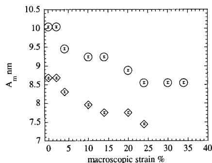
FIGURE 7 The mean center to center distance between microfibrils A_m as a function of macroscopic strain, 45% RH (diamonds), water-filled capillary (circles). For the two humidity conditions, the values of A_m were obtained from the intensity modeling described in the text.
