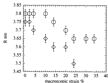
FIGURE 8 The microfibril radius R as a function of macroscopic strain, 45% RH (diamonds), water (circles). For the two humidity conditions the values of R were obtained from the intensity modeling described in the text.
